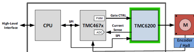
HIGH PERFORMANCE FOC SERVO DESIGN FOR PMSM
